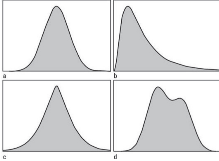
Figure 2: Statistical Distributions
